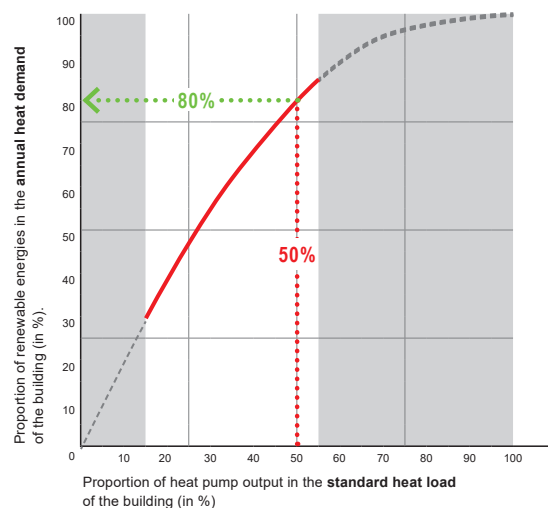
With 50% of the heat load, the Belaria® fit provides 80% of the annual energy consumption. As a result, legal requirements for a high proportion of renewable energies can be met cost-effectively, even in large plants.
